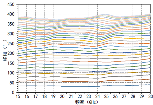
移相VS频率@Pin=-10dBm (Vt=0.5V~16V)
